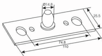
SMALL L PATCH
