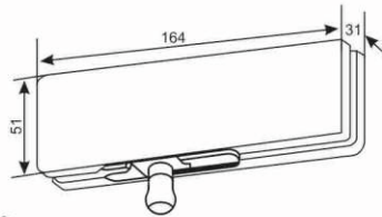
TOP CORNER/OVAR PANEL PATCH
