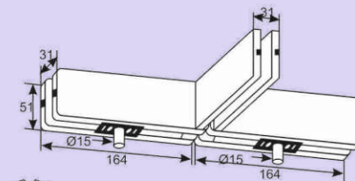
DOUBLE OBER PANEL PATCH FITTING WITH FIN
